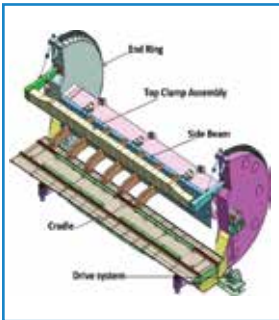
SIDE BEAM WAGON TIPLER
